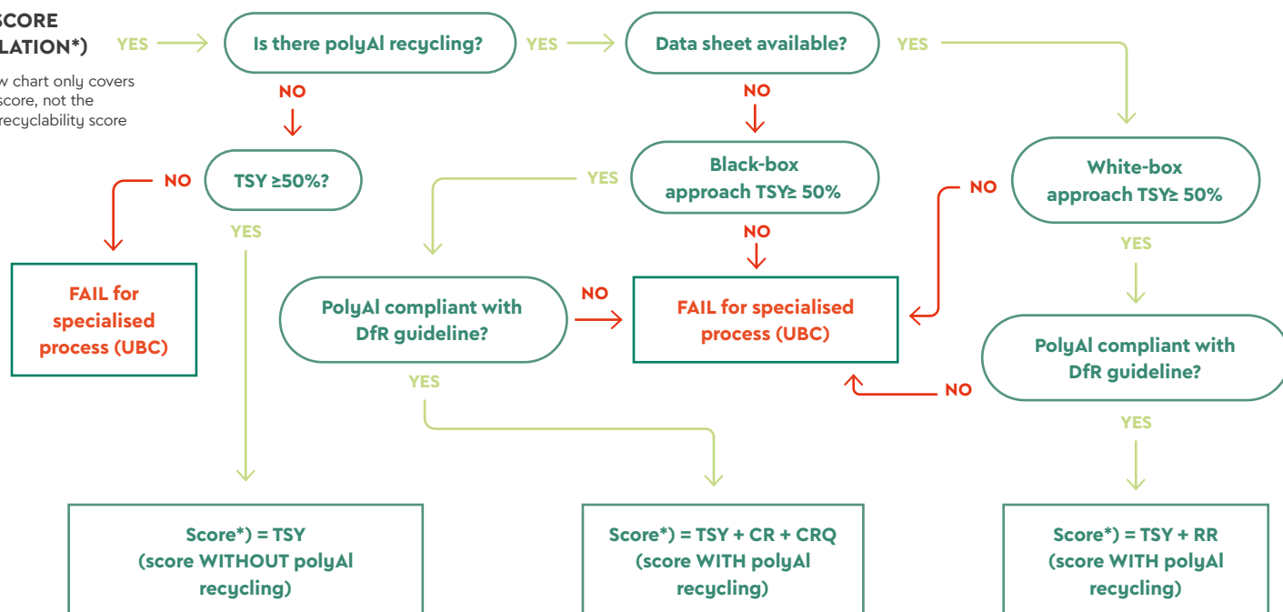
Figure 10. Flow chart for calculating the yield score and when to use the WITH and WITHOUT polyAl recycling options for specialised process (UBC)
