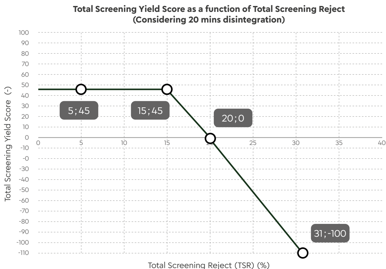
Figure 5. Part I: Total Screening Yield score as a function of Total Screening Reject for 20 min disintegration.
