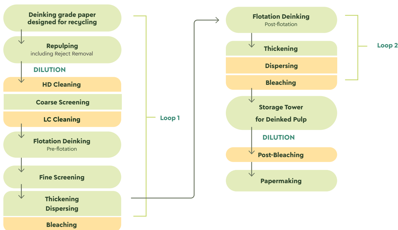
Figure 8. Scheme of the flotation-deinking recycling process
